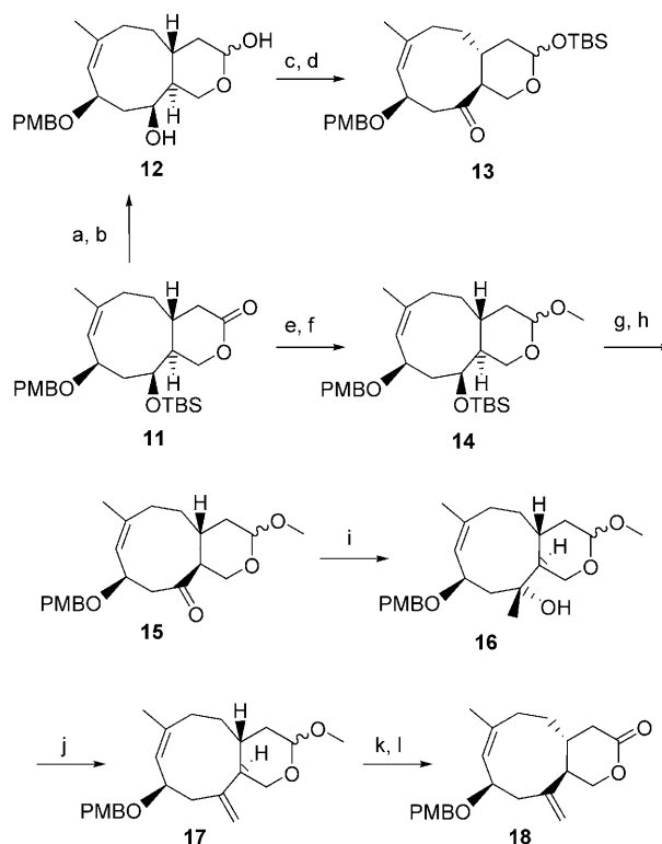
Scheme 4. a) TBAF, THF, 0°C → RT, 85%; b) DIBAL-H, THF, −78°C, 96%; c) TBSOTf, 2,6-lutidine, −78°C, 85%; d) DMP, RT, 88%; e) DIBAL-H, CH 2 Cl 2 , −78°C; f) MeOH, PPTS (5 mol %), RT, 1 h, 73% (two steps, d.r. 1:1); g) TBAF (2 equiv), THF, RT, overnight, 90%; h) TPAP, NMO, 4 Å M.S., CH 2 Cl 2 , 0°C, 1 h, 80%; i) MeMgBr, Et 2 O, −30°C, 30 min, 75%; j) Martin's sulphurane, CH 2 Cl 2 , 0°C → RT, 30 min, 86%; k) 48% aq HF, MeCN/THF (5:1), RT, 2.5 h; l) TPAP, NMO, CH 2 Cl 2 , 4 Å M.S., RT, 30 min, 73% (two steps). TBAF = tetrabutylammonium fluoride, DIBAL-H = diisobutylaluminum hydride, DMP = Dess–Martin periodinane, TPAP = tetrapropylammonium peruthenate, NMO = 4-methylmorpholin- N -oxide, M.S. = molecular sieves.
