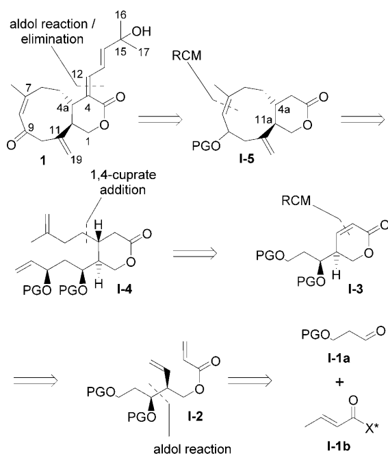
Scheme 1. Retrosynthesis of blumiolide C ( 1 ). PG = protecting group or H. Protecting groups may vary independently.
