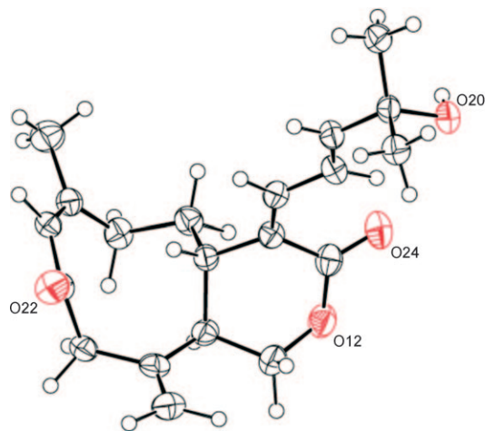
Figure 1. X-ray crystal structure of synthetic blumiolide C ( 1 ). Ellipsoids include 50% of the electron density.
