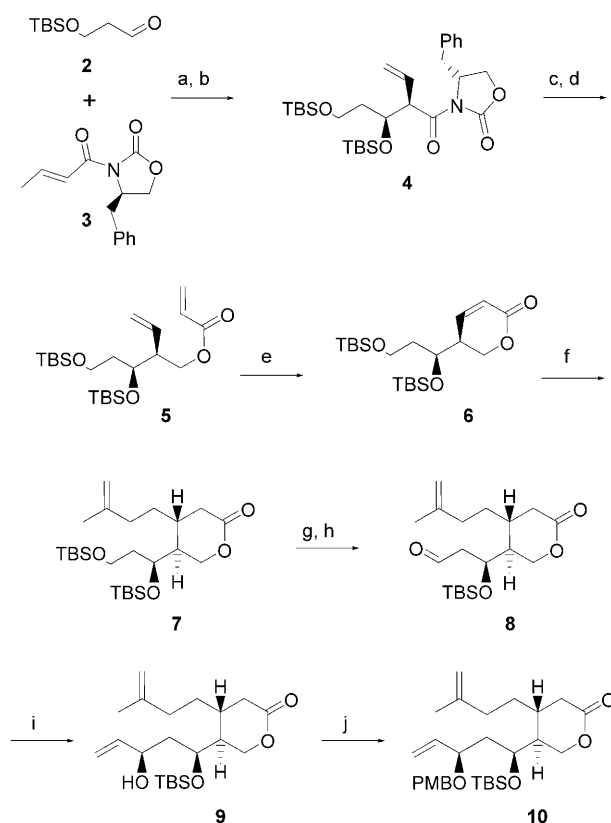
Scheme 2. a) Bu 2 BOTf, Et 3 N, CH 2 Cl 2 , –78 °C → RT, 1.5 h, 95 %; b) TBSOTf, 2,6-lutidine, CH 2 Cl 2 , 0 °C, 1 h, 93 %; c) LiBH 4 , MeOH (1 equiv), Et 2 O, 0 °C → RT, 1.5 h, 77 %; d) CH 2 =CHC(O)Cl, Et 3 N, DMAP, CH 2 Cl 2 , 0 °C, 1 h, 75 %; e) Grubbs II, CH 2 Cl 2 , reflux overnight, 92 %; f) CH 2 =C(CH 3 )CH 2 CH 2 MgI, CuI, Et 2 O, –78 °C, 90 %; g) CSA, MeOH/CH 2 Cl 2 (1:1), 0 °C, 30 min, 90 %; h) DMSO, (COCl) 2 , Et 3 N, –78 °C, 93 %; i) CH 2 =CHMgCl, ZnCl 2 , THF, –30 °C, 18 h, 62 %, d.r. 5:1; j) PMBOC(=NH)CCl 3 , cyclohexane, PPTS (3 mol %), 0 °C → RT, 20 h, 68 %. Tf = trifluoromethanesulfonyl, DMAP = 4-dimethylaminopyridine, CSA = (+)-camphorsulfonic acid, DMSO = dimethylsulfoxide, PMB = para -methoxybenzyl, PPTS = pyridinium p -toluenesulfonate.
