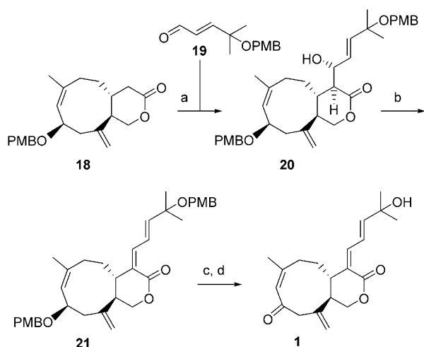
Scheme 5. a) LDA (3 equiv), THF, -78^{\circ}\text{C} , then 19 , 2 h, 50%; b) neat DCC, \text{CuCl}_2 , RT, overnight, 90%; c) DDQ, \text{CH}_2\text{Cl}_2 /phosphate buffer (20:1), RT, 68%; d) DMP, \text{CH}_2\text{Cl}_2 , RT, 1 h, 85%. LDA = lithiumdiisopropylamide, DCC = N,N' -dicyclohexylcarbodiimide, DDQ = 2,3-dichloro-5,6-dicyano-1,4-benzoquinone.
