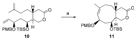
Scheme 3. a) [ 10 ] = 1.5 mM, Hoveyda–Grubbs II catalyst, 50 mol %. For other conditions see Table 1.
